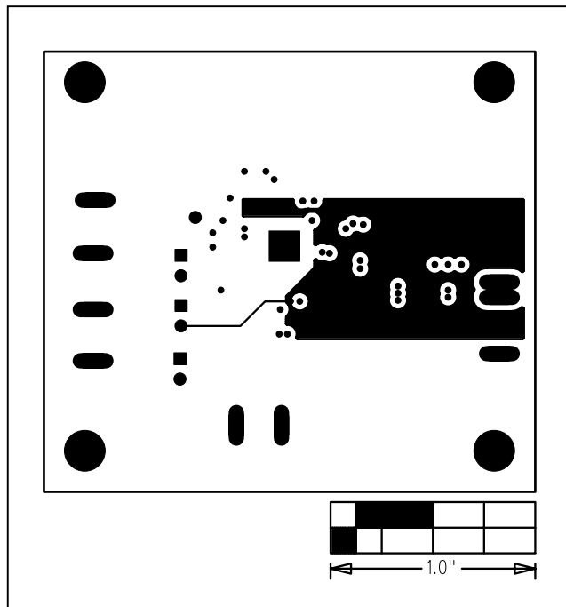
Figure 5. MAX15015A EV Kit PCB Layout—Power Layer 3
