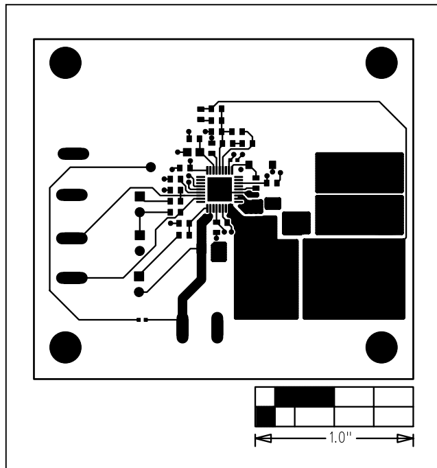
Figure 3. MAX15015A EV Kit PCB Layout—Component Side
